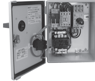
Painted Steel, Type 4 / 12 Enclosure
