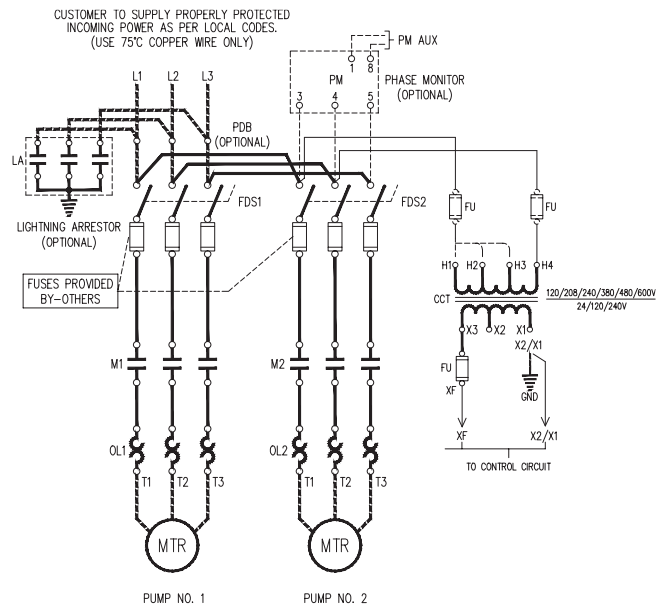
PUMP NO. 1 PUMP NO. 2
