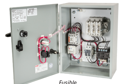
Fusible Combination Starter
