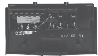
CA5 Feeder Group - rear view (typical)
