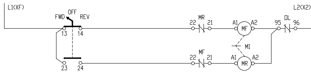
FORWARD OFF REVERSE SEL. SW.
