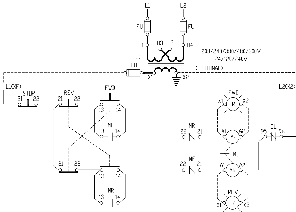
FORWARD STOP REVERSE PB
