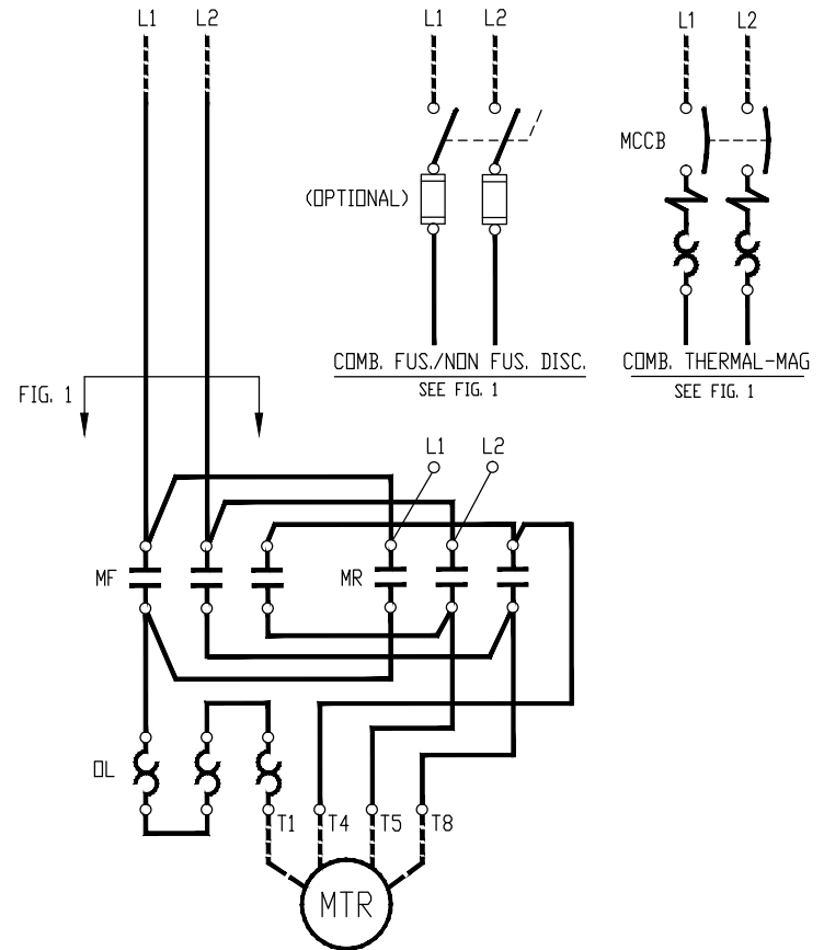
1-PH 4-LEAD REPULSION INDUCTION MOTOR
